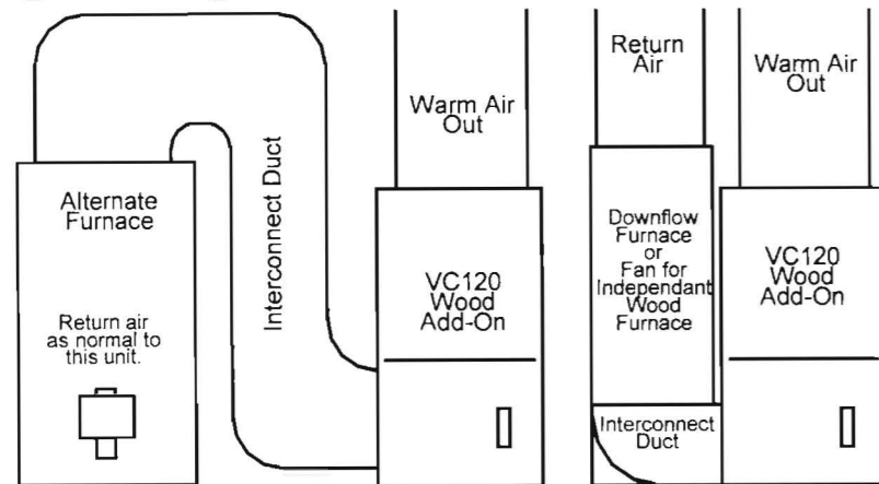
TYPICAL INSTALLATIONS
