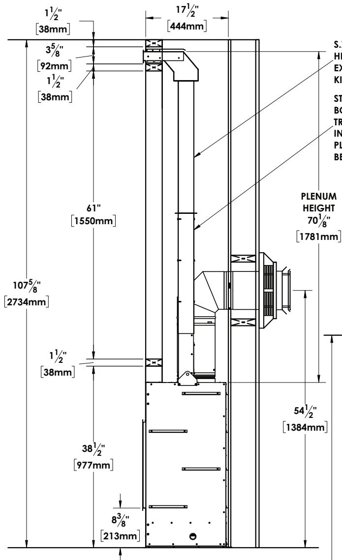
Fig. 5d Typical 9ft Ceiling - Floor Installation
