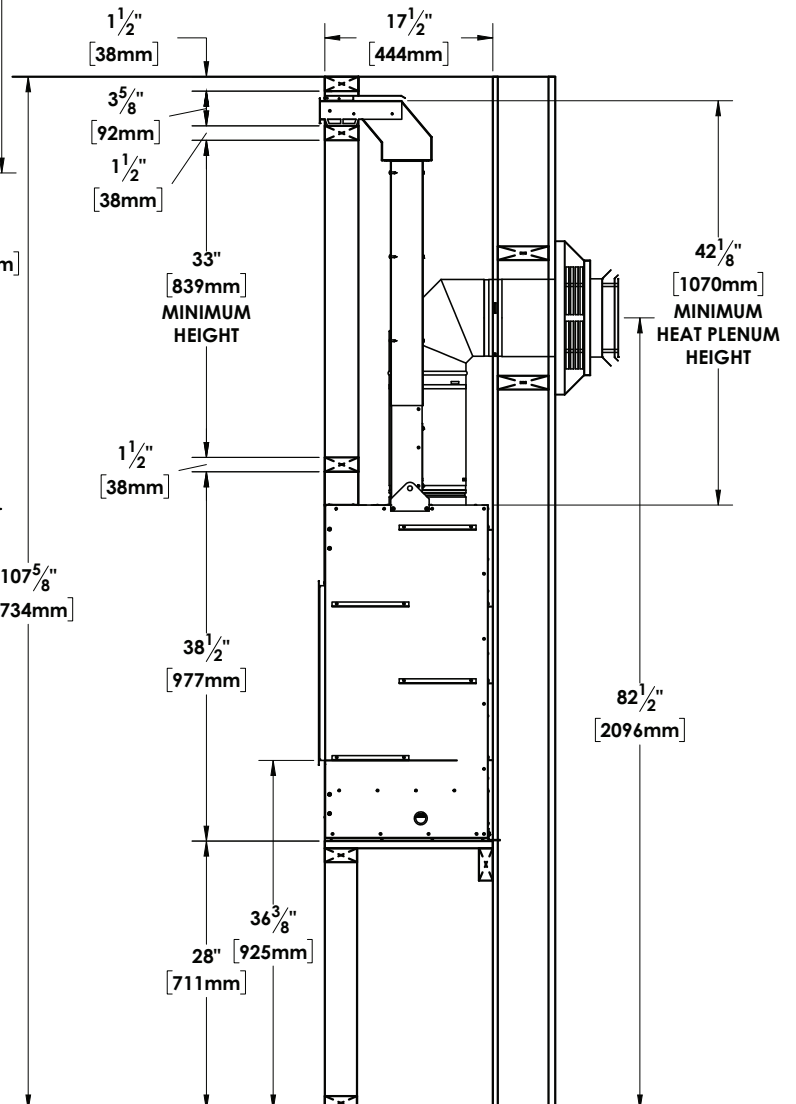
Fig. 5e Typical 9ft Ceiling - Raised Installation
