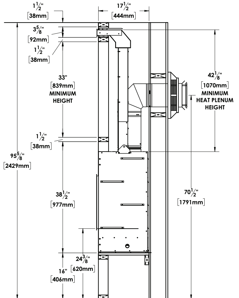
Fig. 5c Typical 8ft Ceiling - Raised Installation
