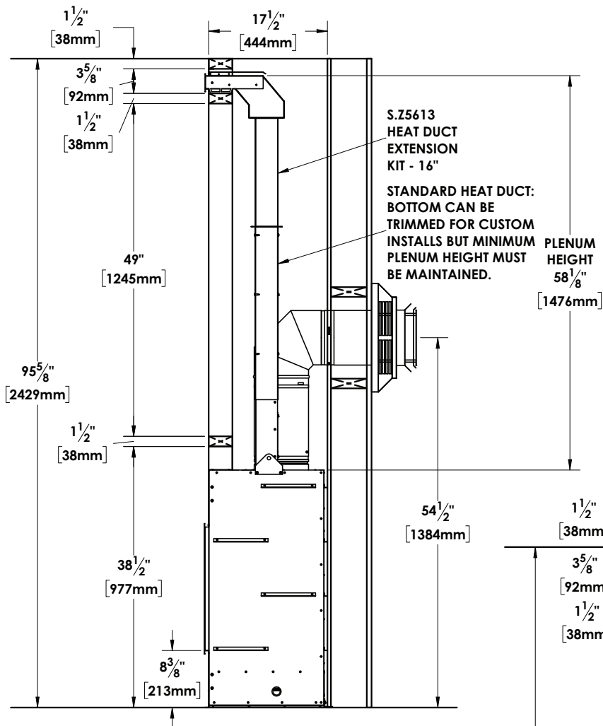
Fig. 5b Typical 8ft Ceiling - Floor Installation
