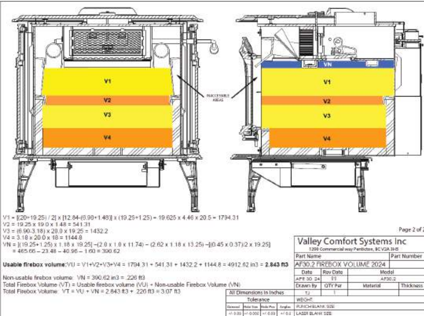
Figure 6 - Firebox Volume - Calculations
