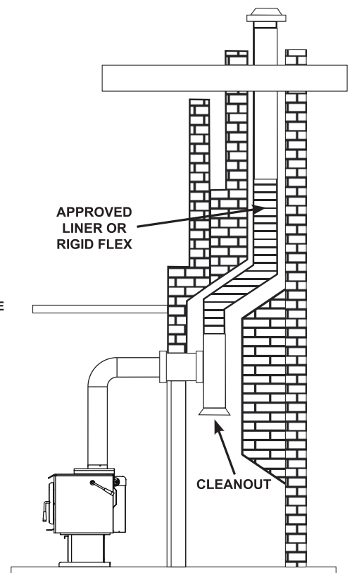
Blaze King Recommend Installation
