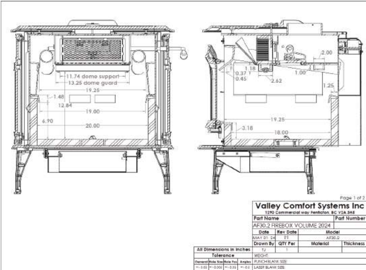
Figure 5 - Firebox Volume - Dimensions
