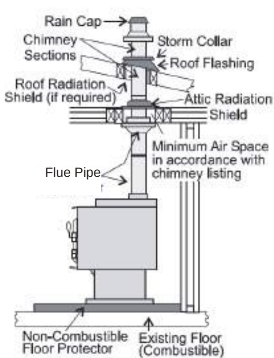
Prefab Chimney Through Ceiling Installation
