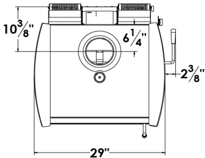
Figure 10 - Over-all Dimensions of model variant CH30.2
