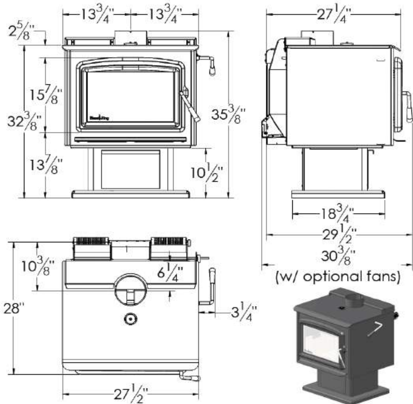
Figure 8 - Over-all Dimensions of model variant SC30.2 (with Pedestal Option)
