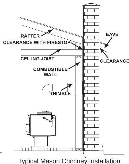
Blaze King Recommend Installation
