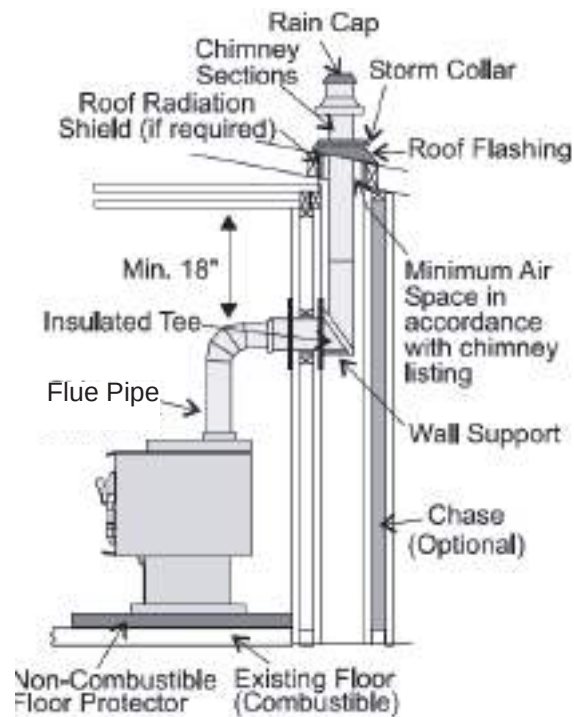
Prefab Chimney Exterior Installation
