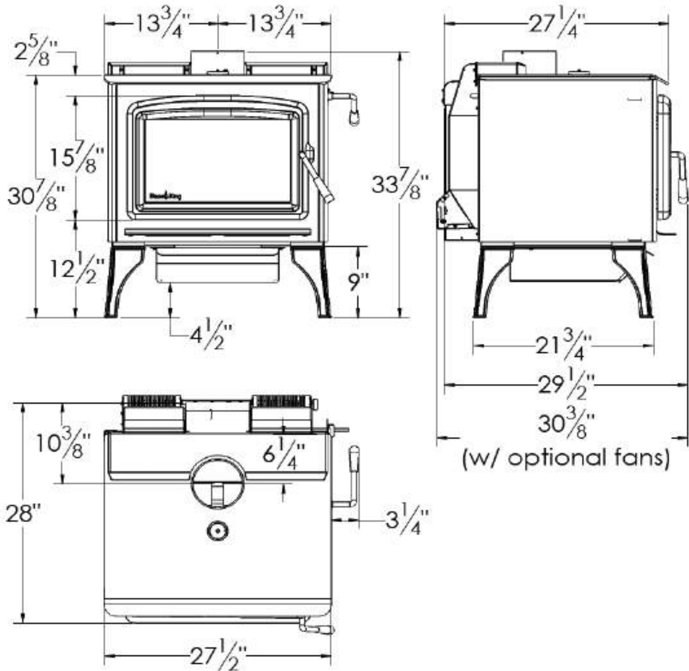
Figure 9 - Over-all Dimensions of model variant SC30.2 (with Leg Option)
