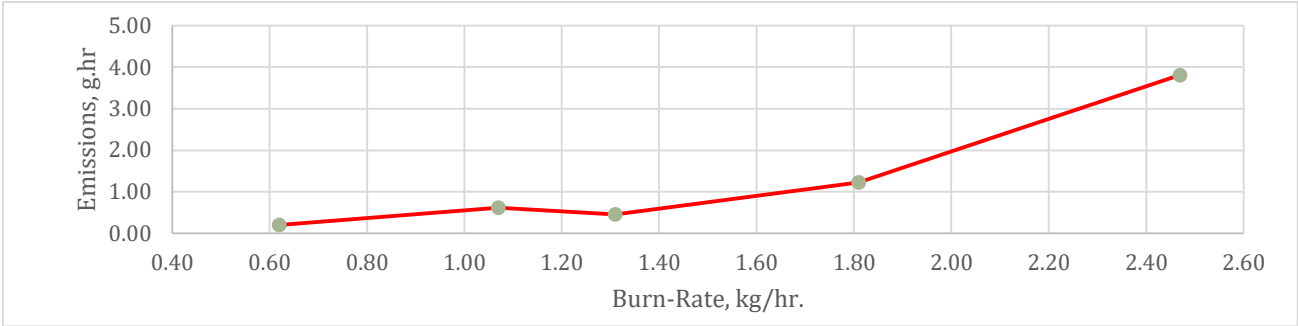
Figure 1 - Emissions Plot by Burn-Rate
